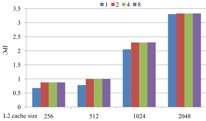
Fig. 11. IPC values of bzip2 for different configurations of L2 cache size and L2 MSHR number.
