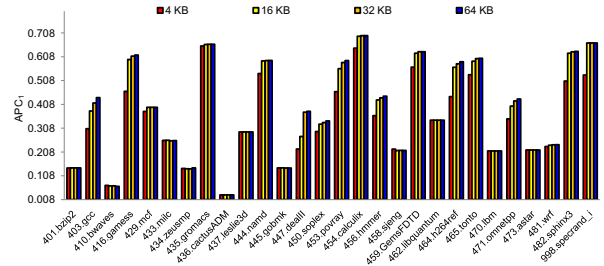
Fig. 6. APC_1 of the applications running on cores with different L1 data cache size
